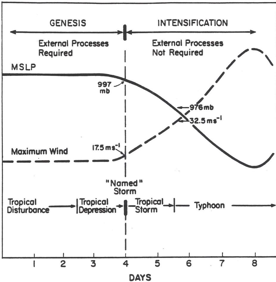
Figure 1.1: Depiction of typical genesis and intensification periods and their characteristics.
