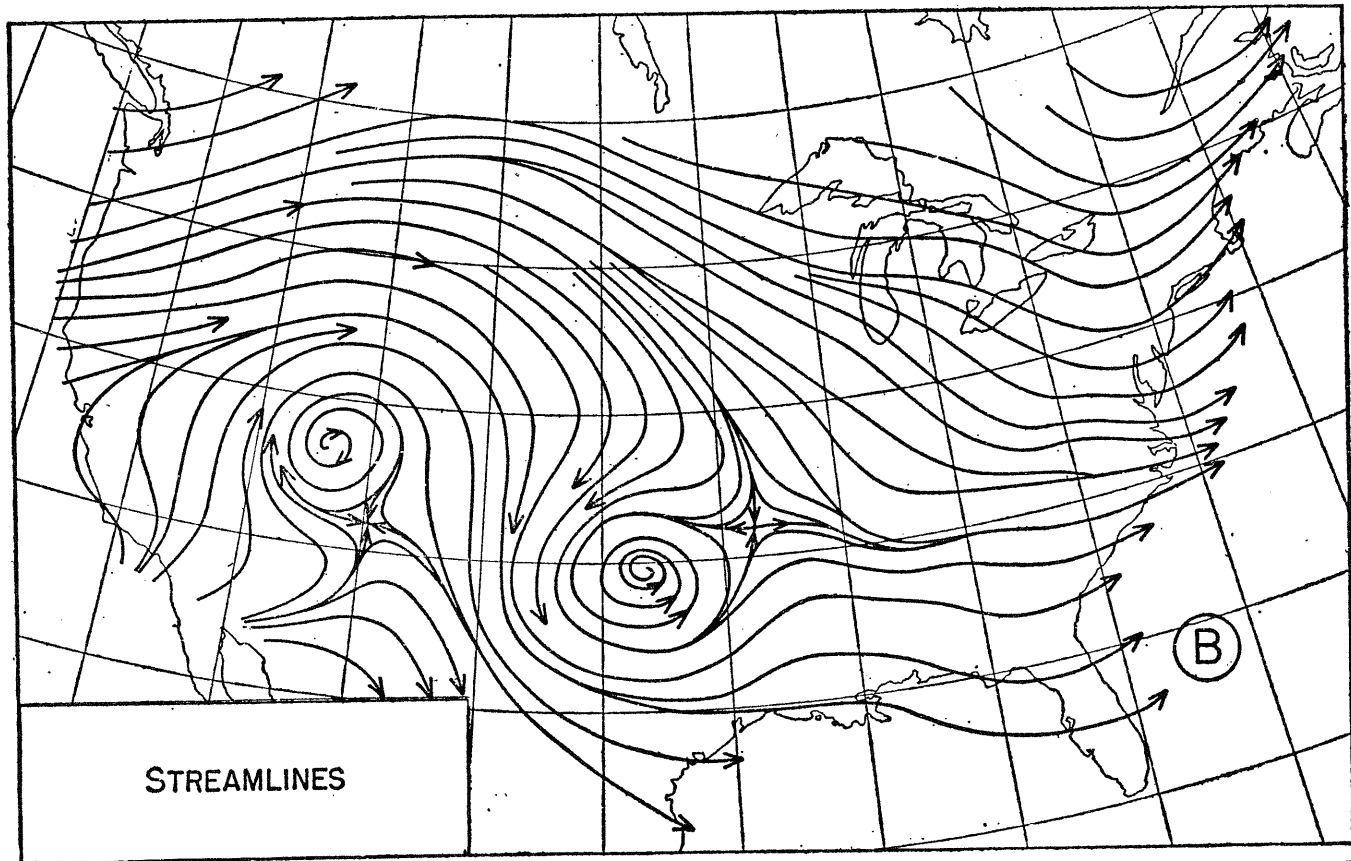
FIG. 2.2.2. Illustrating the construction of streamlines. A, the line segments and principal isogons; B, the streamlines. The charts represent the conditions at the 18,000-ft level on June 5, 1950, 1500 GMT. (Analysis by Col. A. F. Gustafson.)
